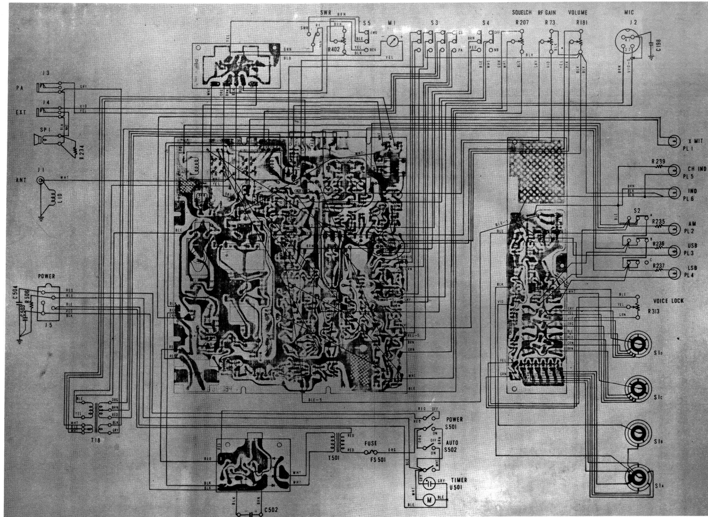
WIRING DIAGRAM COBRA 135(A) FIG. 23
